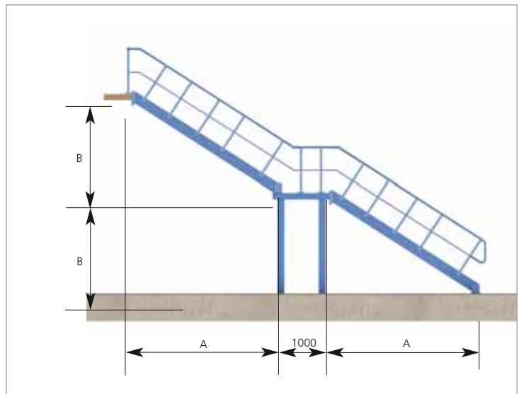
Continuous stairway with a landing
