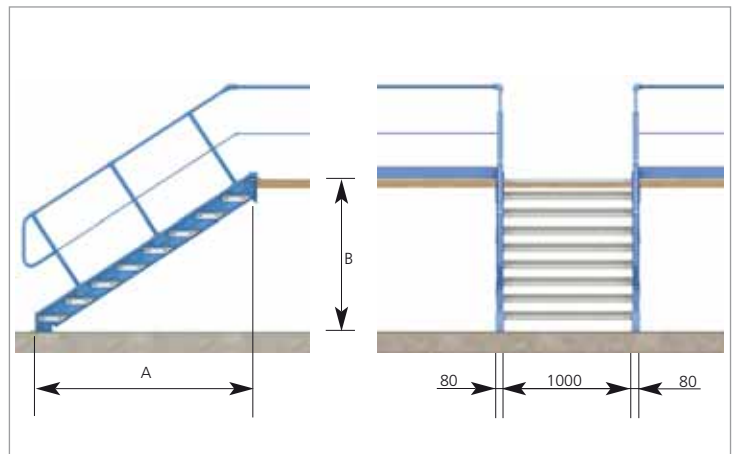
Stairway without a landing
